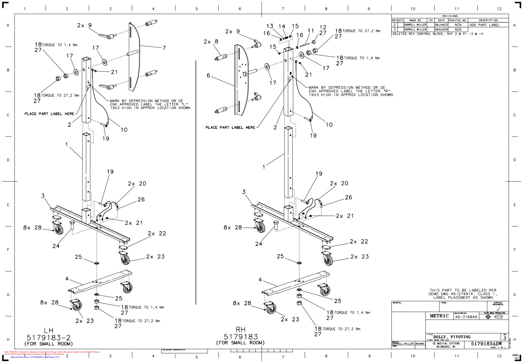
Figure 5-2 Dolly, Pivoting, Small Room (5179183 sheet 1, rev 3)
